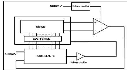
Fig .2. Basic overview Architecture of shrew x2
