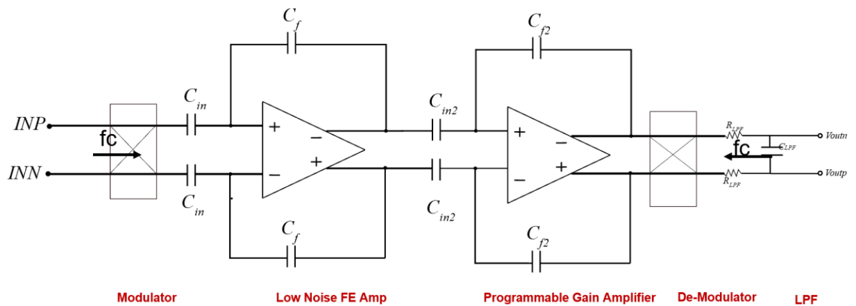
Figure 6: New LNA Architecture
